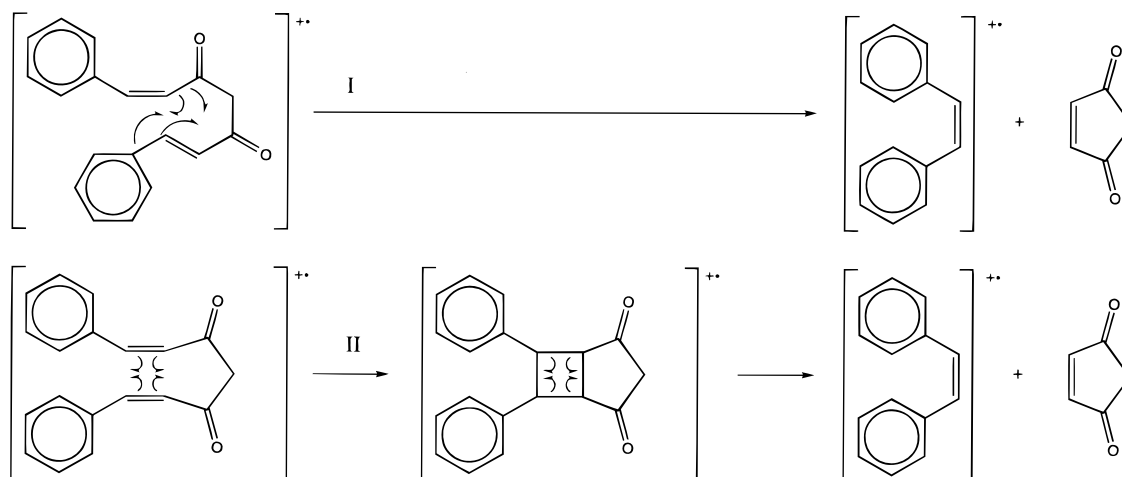
Scheme 3
