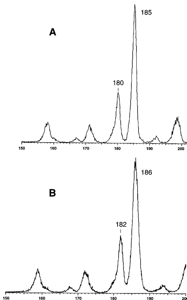
Figure 2. Partial MIKE mass spectra of the molecular ions of (A) 14 and (B) 14\text{-}^{13}\text{C}_2 .
