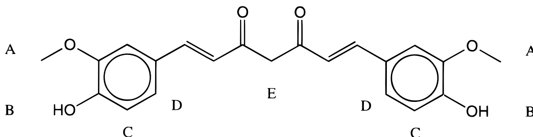
Figure 1. Structure of curcumin with indication of substituent positions.
