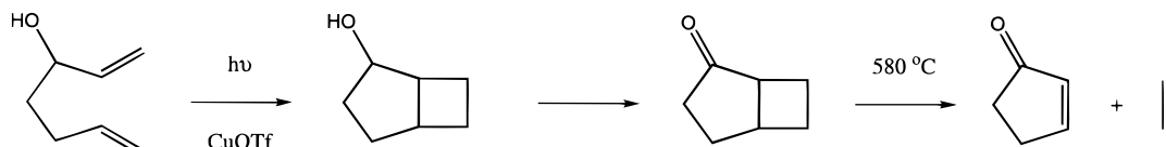
Scheme 4
